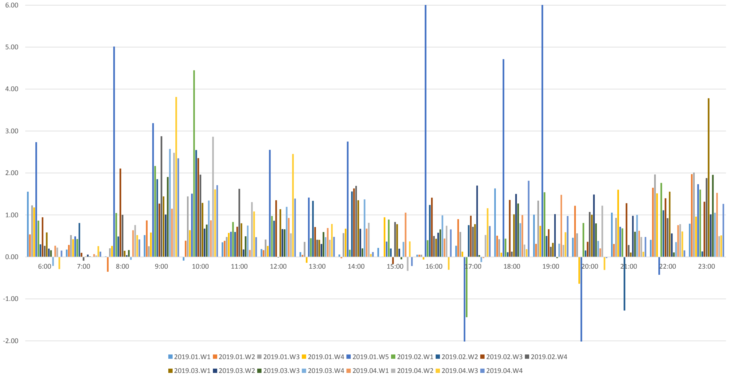
501 Queen Difference in Average Weekly Headways Westbound at Silver Birch vs Coxwell Jan-Apr 2019
