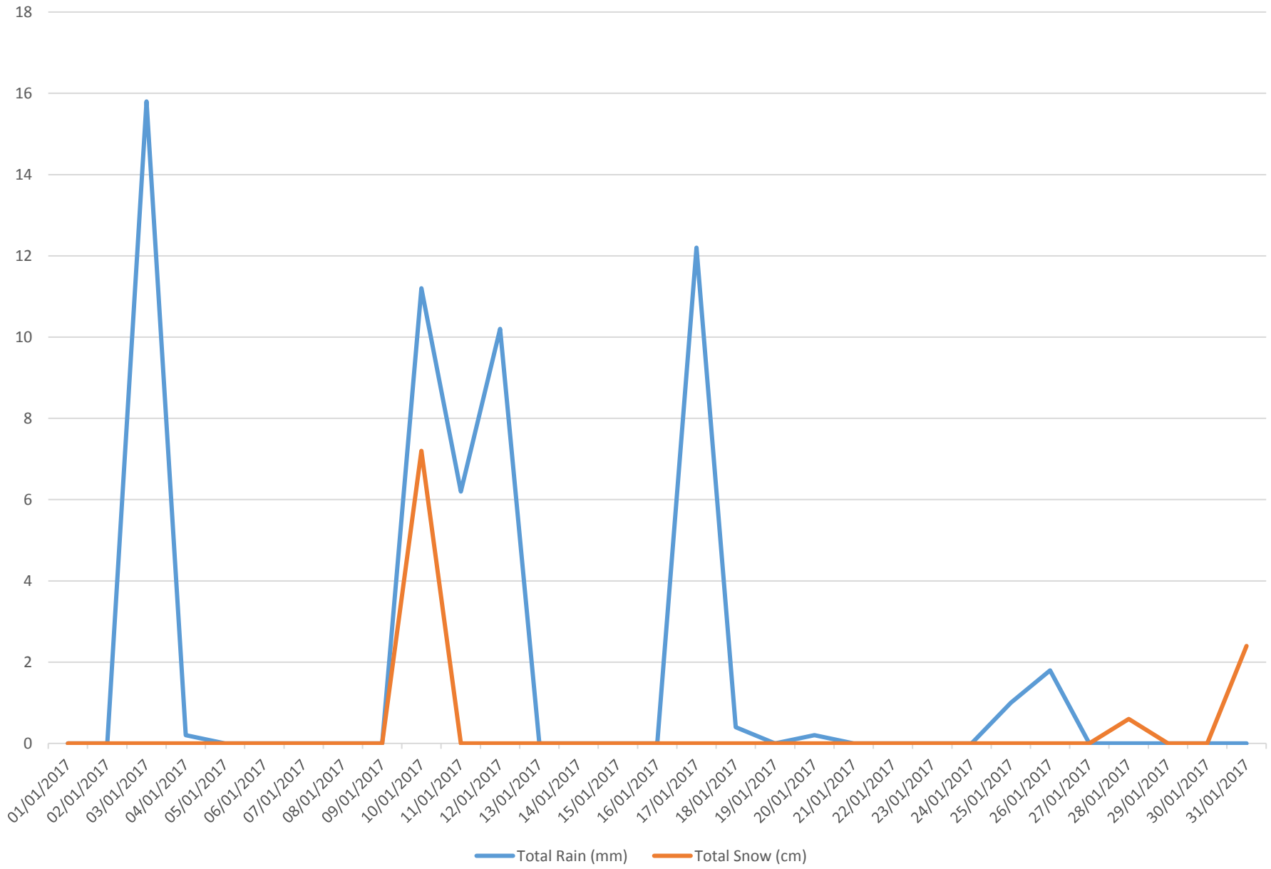
2017 Precipitation at Toronto (YYZ)
