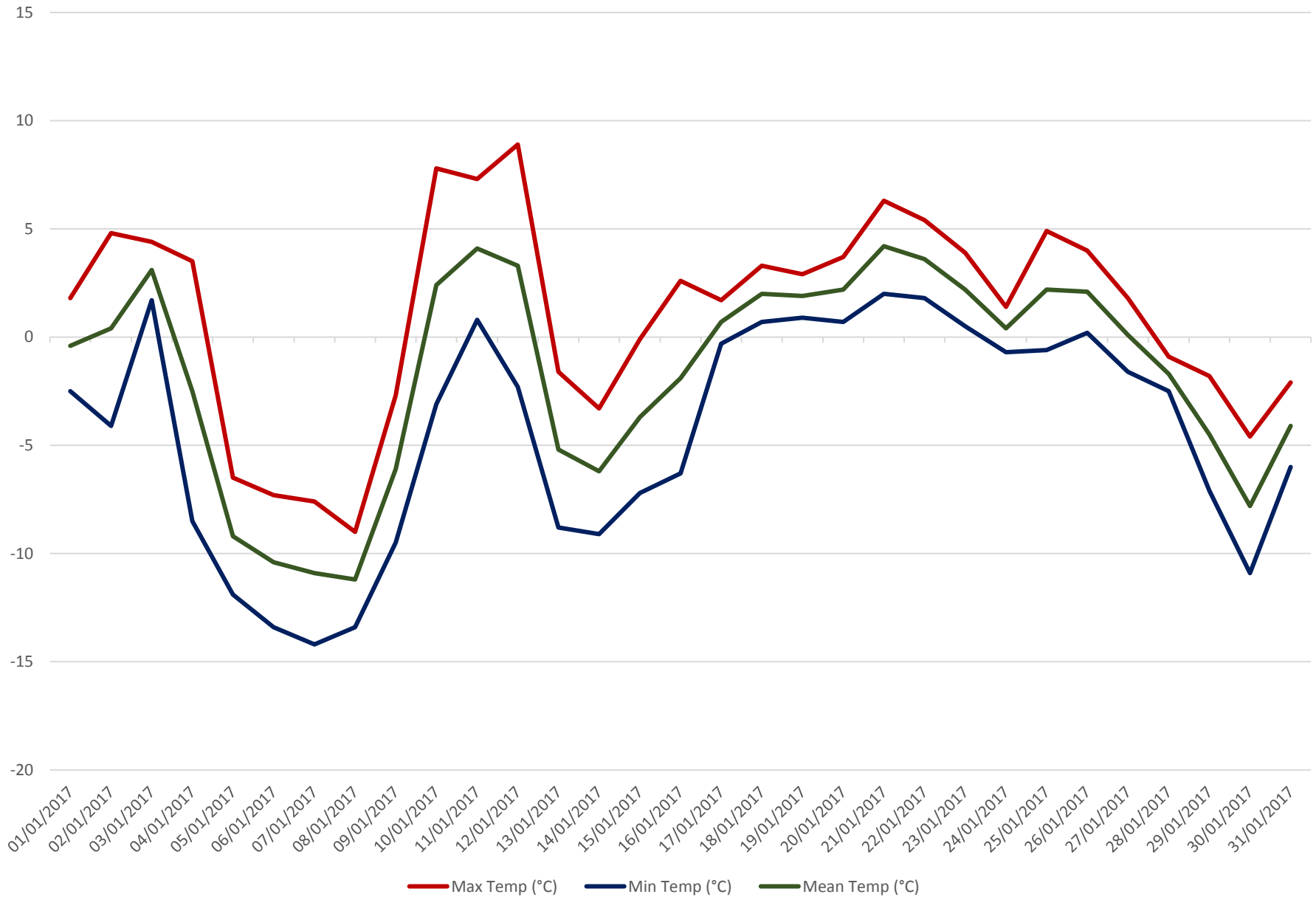
2017 Temperatures at Toronto (YYZ)
