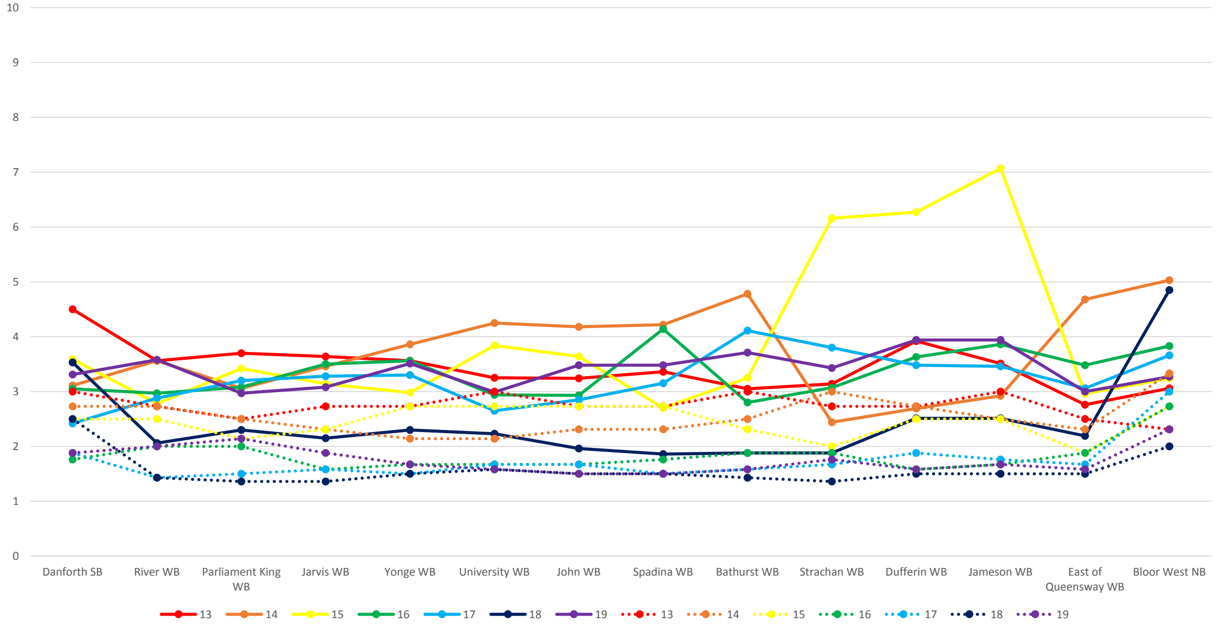
504 King Rider Wait Times (Solid) and Smoothed Half-Headways (Dotted) 1 Nov 2016 Westbound
