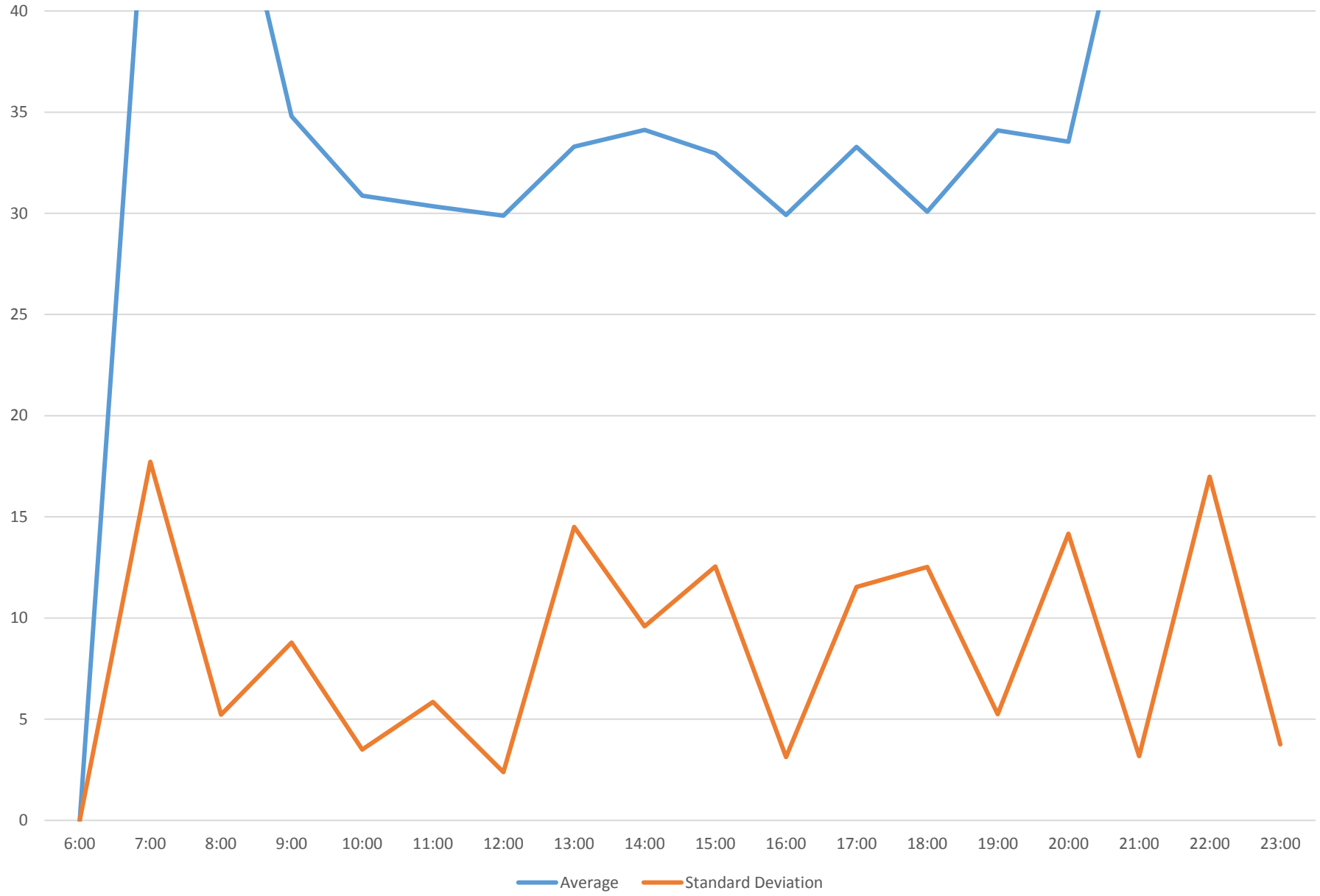
96 Wilson Headways at S of Carrier Loop Eastbound September 2015 Sunday Statistics
